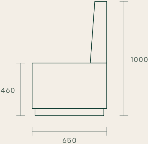
SIDE
