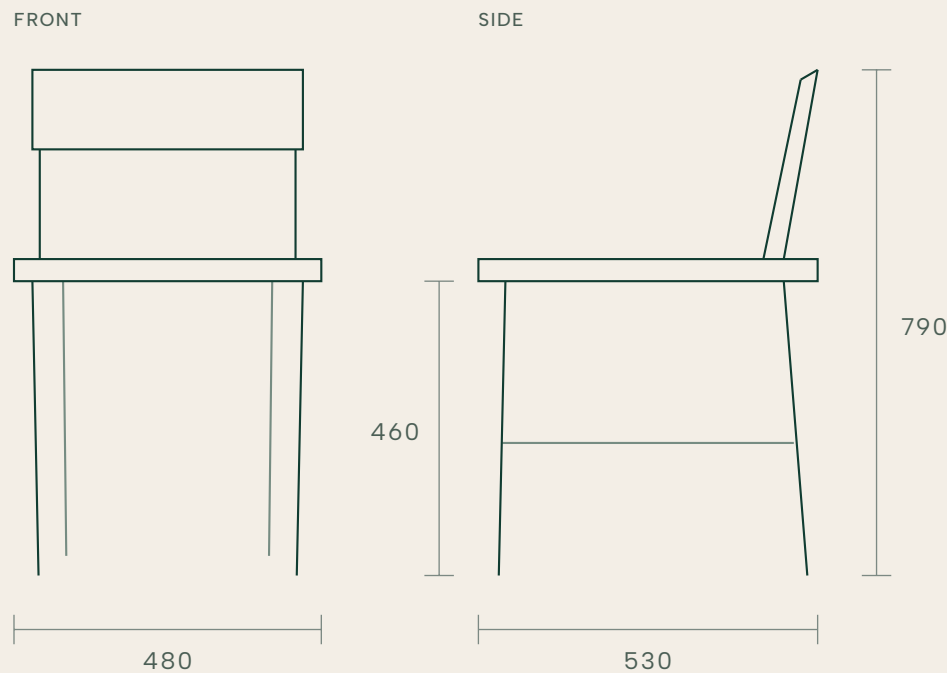
Front and side elevation — schematic, generated from the catalogue dimensions. CAD and 3D files on request.
