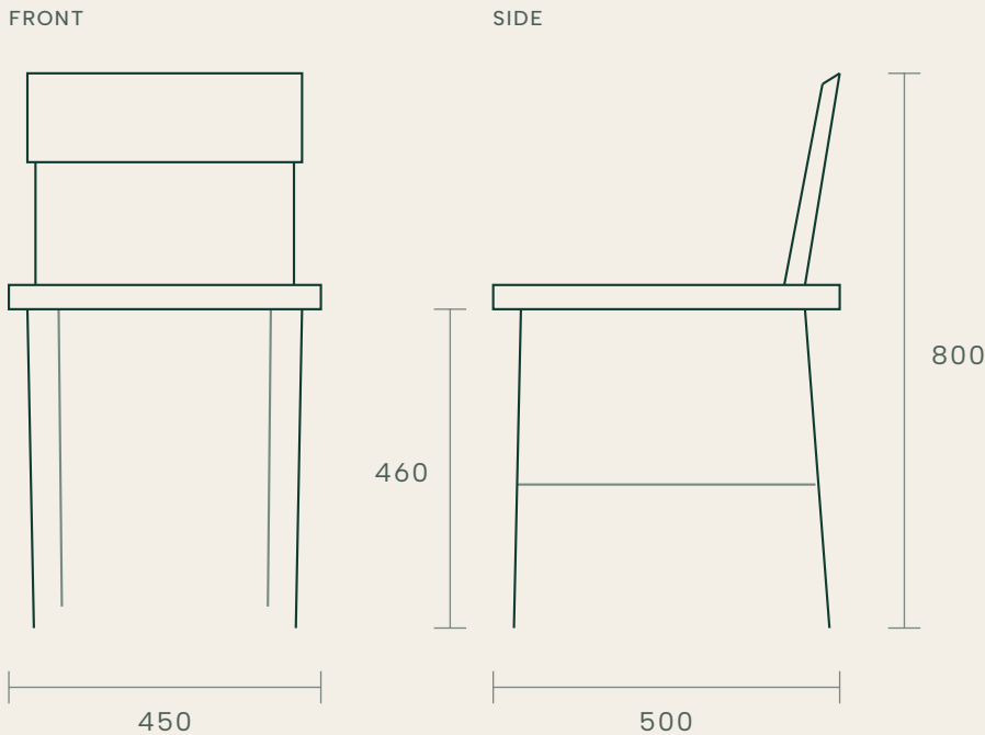
Front and side elevation — schematic, generated from the catalogue dimensions. CAD and 3D files on request.
