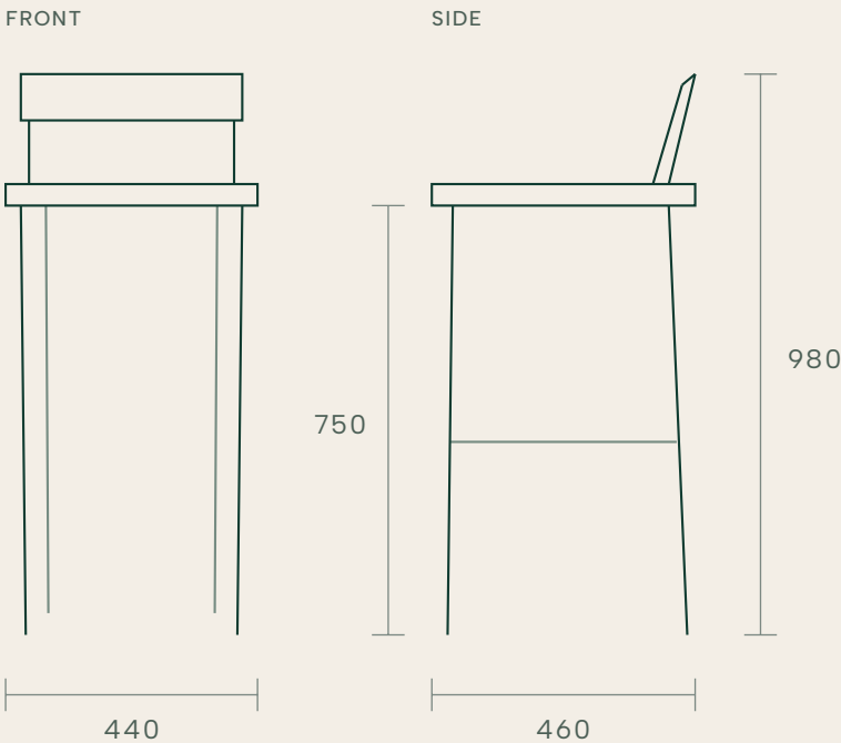
Front and side elevation — schematic, generated from the catalogue dimensions. CAD and 3D files on request.
