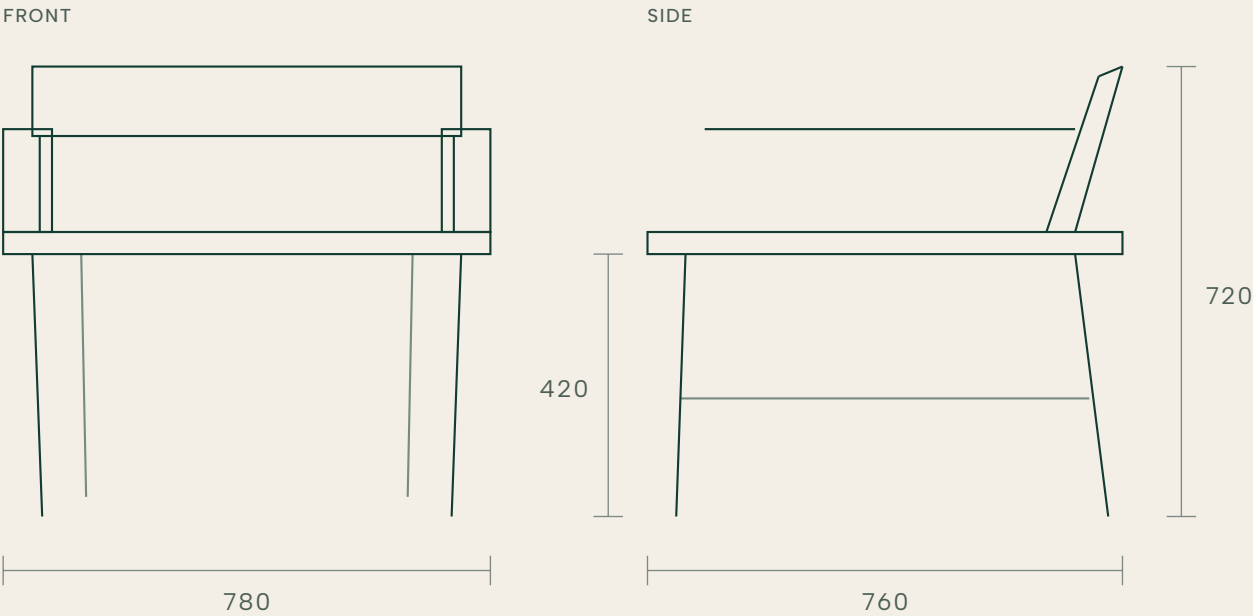
Front and side elevation — schematic, generated from the catalogue dimensions. CAD and 3D files on request.
