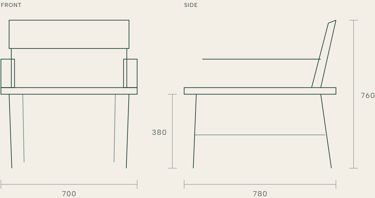
Front and side elevation — schematic, generated from the catalogue dimensions. CAD and 3D files on request.
