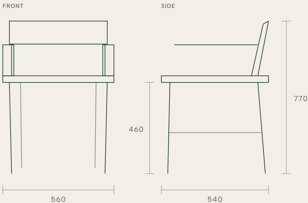
Front and side elevation — schematic, generated from the catalogue dimensions. CAD and 3D files on request.
